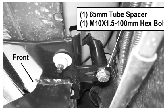
(Fig 3) Driver Front Mounting Bracket Installation
