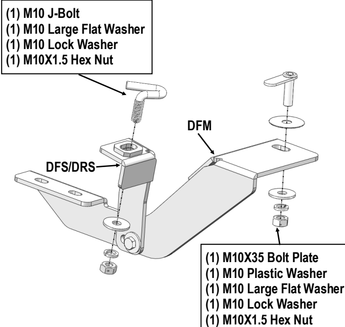
(Fig 5) Driver Side Front Mounting Bracket Installation
