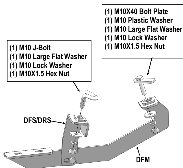
(Fig 13) Driver Side Rear Mounting Bracket Installation
