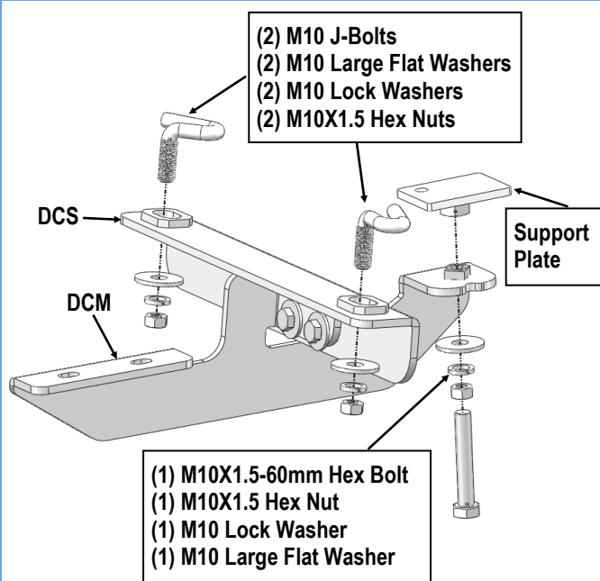
(Fig 9) Driver Side Center Brackets Installation
