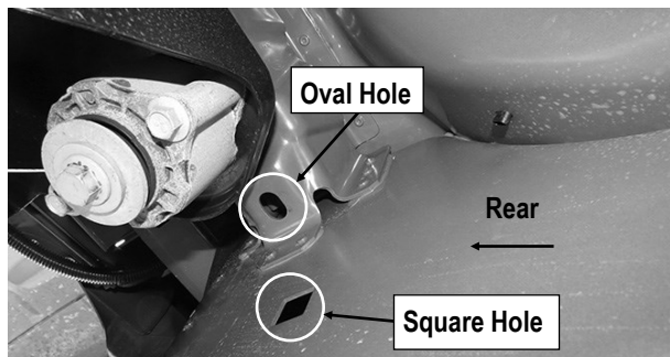
(Fig 6) Driver Side Rear Mounting Location
