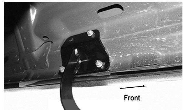
(Fig 7) Driver Front Mounting Bracket Installed
