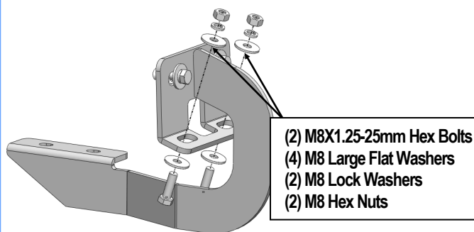
(Fig 4) Driver Front Mounting Bracket Installed to Pinch Weld
