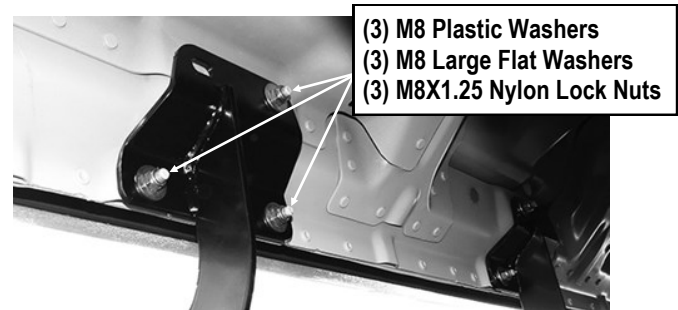
(Fig 4) Passenger Front Mounting Bracket Installed (Example)
