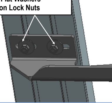
(Fig 22) Running Board Installed Onto the Mounting Bracket
