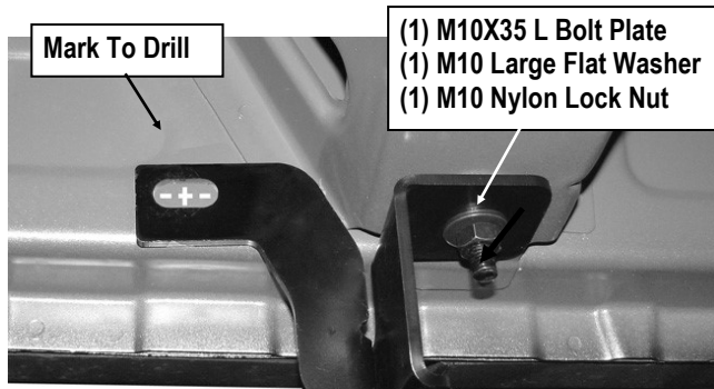
(Fig 5) Driver Side Center Bracket Assembly
