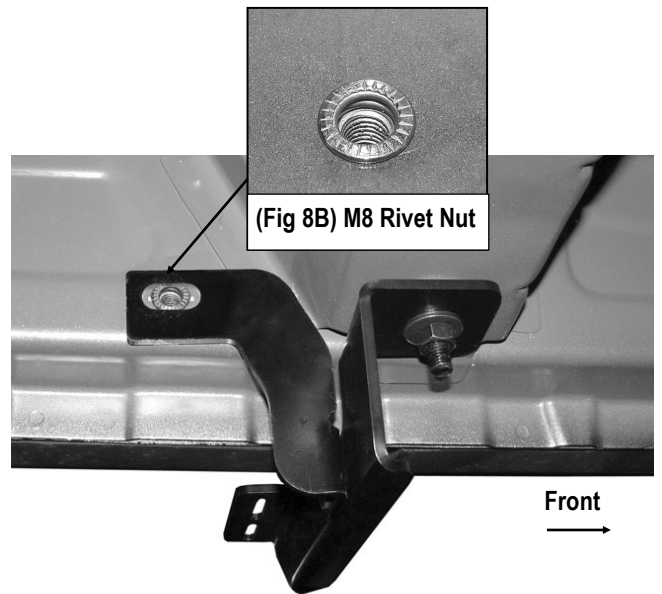
(Fig 8A) Driver Side Center Bracket Installation (2007-11)
