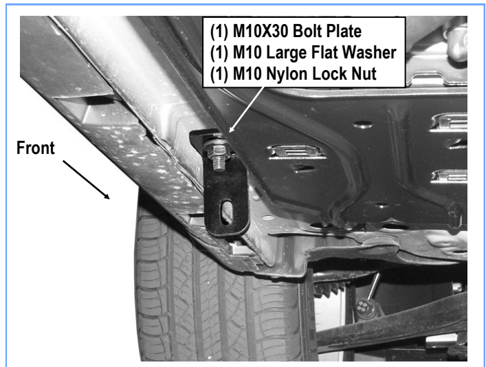
(Fig 2) Driver Front Support Bracket Installed
