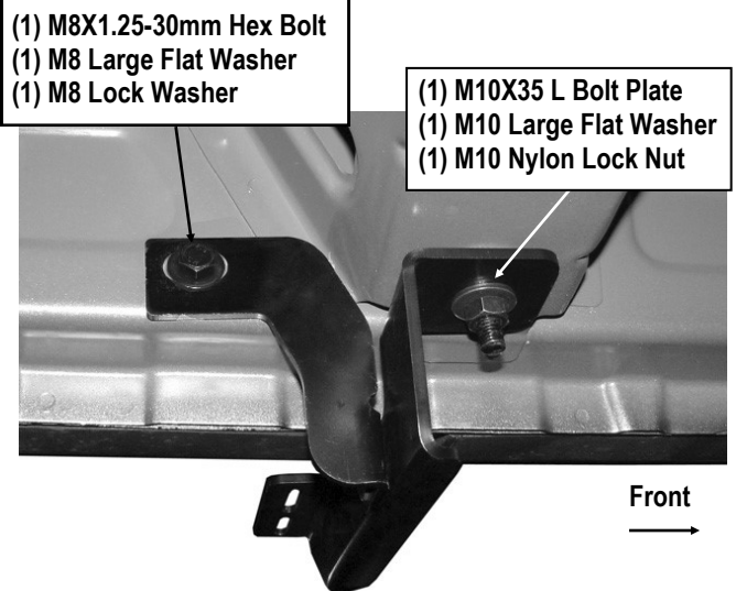
(Fig 8C) Driver Side Center Bracket Installed (For 2007-2011 Models)
