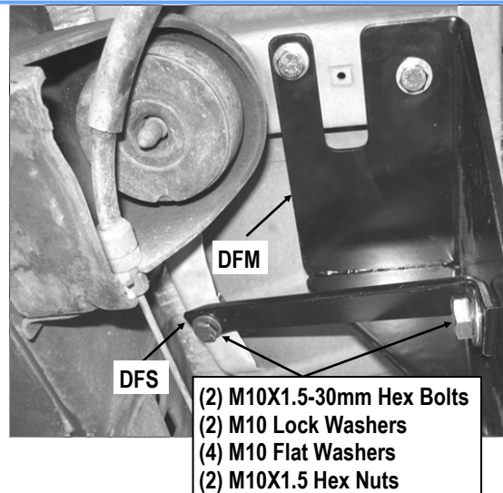
(Fig 3) Driver Front Support Bracket Installed
