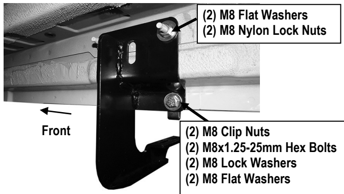
(Fig 11) Passenger Side 2nd Mounting Bracket Installation
