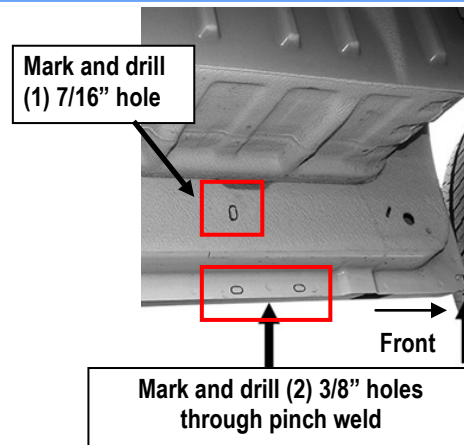
(Fig 16) Driver Side Front Mounting Bracket Location
