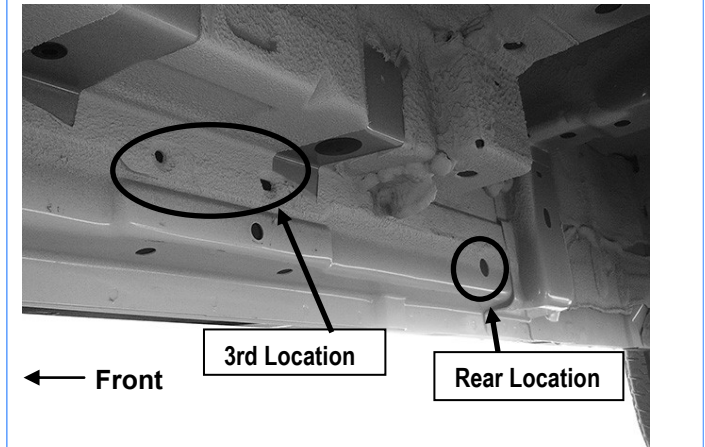
(Fig 13) Passenger Side 3rd/Rear Mounting Bracket Location
