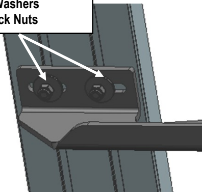
(Fig 15) Running Board Installed Onto Driver Center Mounting Bracket
