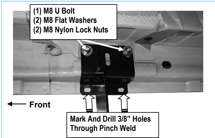
(Fig 10) Passenger Side 2nd Mounting Bracket Installation
