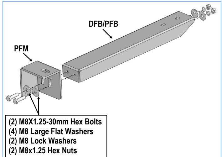
(Fig 3) Passenger Side Front Brackets Assembly
