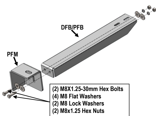
(Fig 3) Passenger Side Front Brackets Assembly
