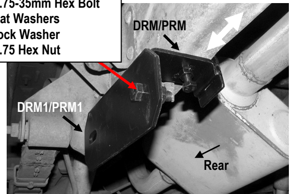
(Fig 6) Passenger Rear Mounting Bracket 1 Installation
