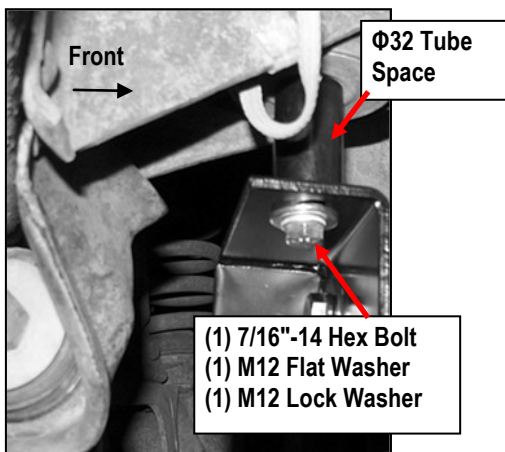
(Fig 4) Passenger Front Mounting Bracket (PFM) Installation
