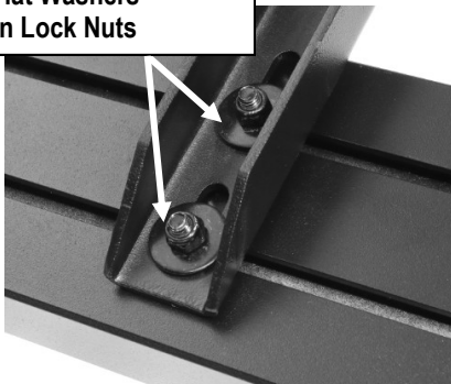
(Fig 12) Running Board Installed Onto Driver Center Mounting Bracket
