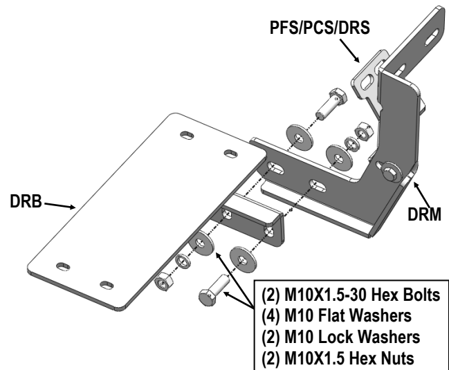
(Fig 18) Driver Side Rear Bar Bracket Assembly
