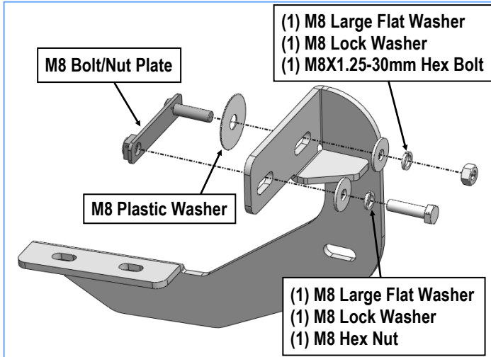
(Fig 9) Driver Front Mounting Bracket Installation
