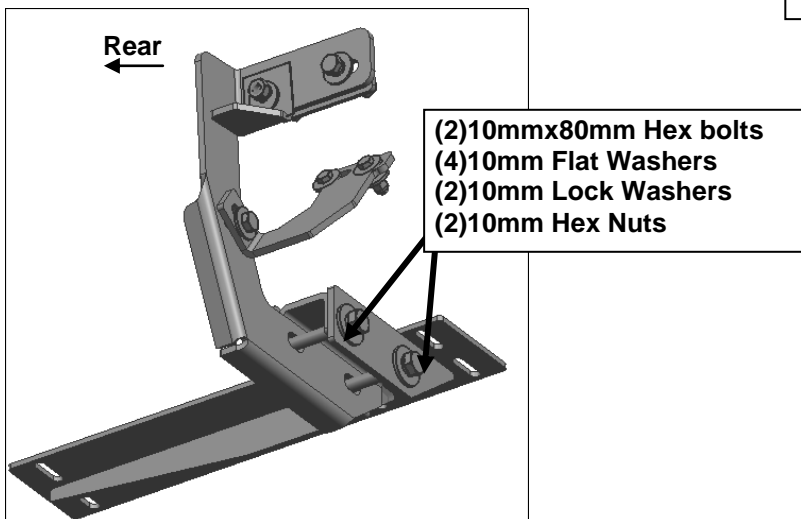
(Fig 17) Driver/Left rear Lower Mounting Bracket assembly
