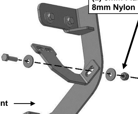
(Fig 9) Attach Driver/Left front Support Bracket to front facing side of Mounting Bracket
