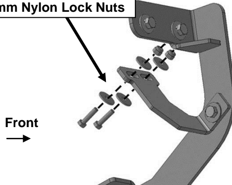
(Fig 10) Attach Support Bracket to back of pinch weld (models with factory holes in pinch weld only)
