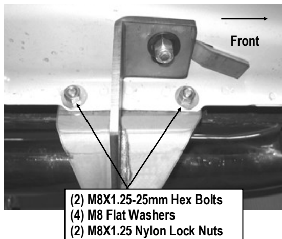
(Fig 3) Driver Front Mounting Bracket Installed
