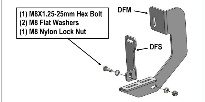
(Fig 2) Driver Front Mounting Bracket (DFM) and the Driver Front Support Bracket (DFS) Assembly
