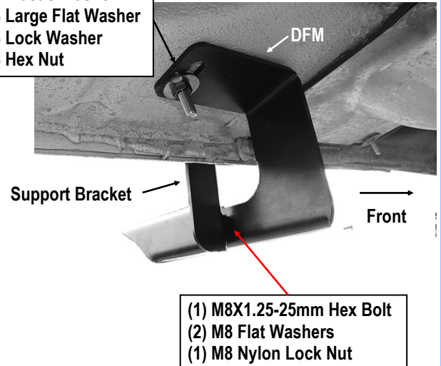
(Fig 5) Driver Rear Mounting Bracket Installation
