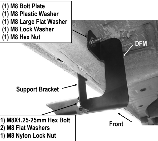
(Fig 11) Passenger Side Front Bracket Installation
