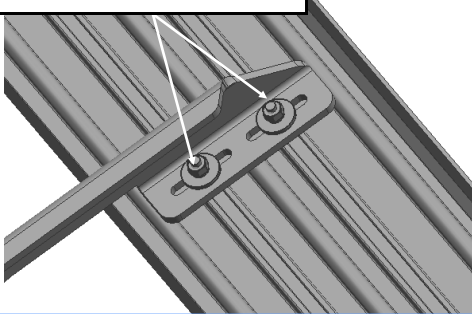
(Fig 7) Running Board Installed Onto Mounting Bracket (Example)
