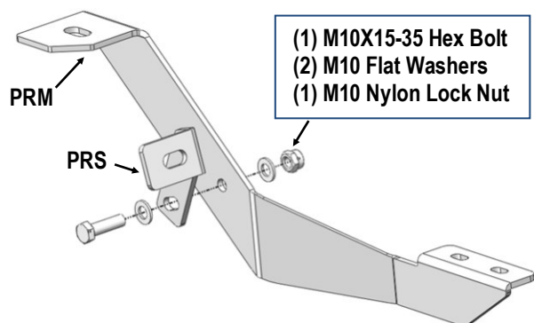
(Fig 9) Passenger Rear Mounting Brackets Assembly
