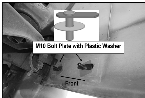
(Fig 2) M10 Bolt Plates with M10 Plastic Washers (on Passenger Side Front Mounting Location)
