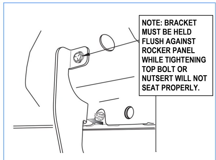
(Fig 4) Re-attach Trim Panel As Shown
