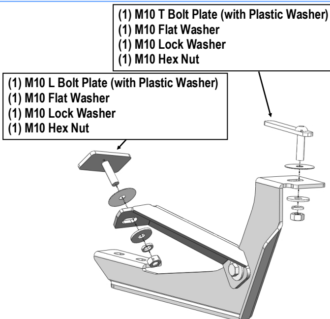
(Fig 13) Driver Side Center Brackets Installation
