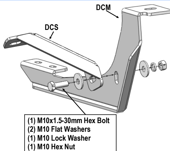
(Fig 12) Driver Side Center Brackets Assembly
