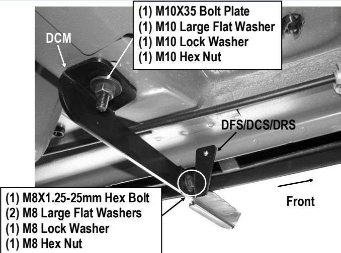
(Fig 6) Driver Side Center Brackets Installed
