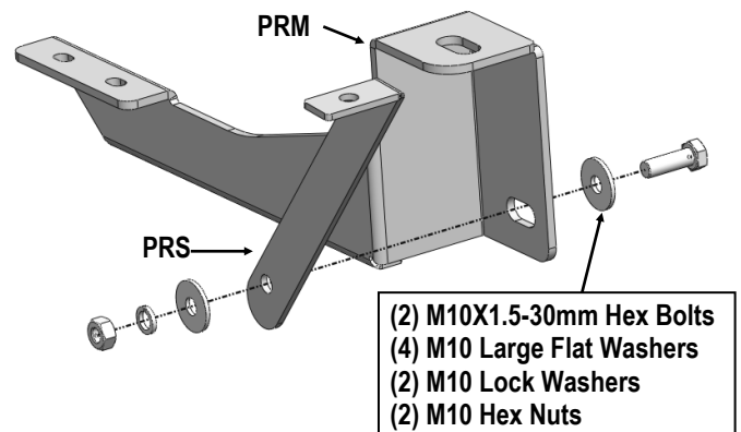
(Fig 3) Passenger Side Rear Brackets Assembly
