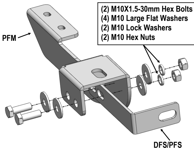
(Fig 1) Passenger Side Front Brackets Assembly
