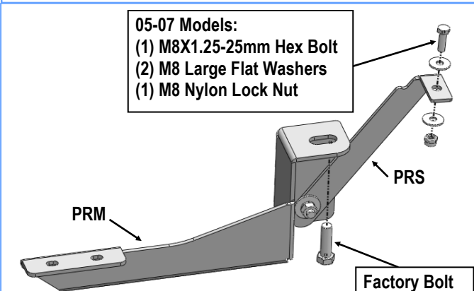
(Fig 4) Passenger Side Rear Brackets Installation (05-07 Models)
