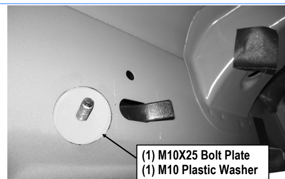
(Fig 9) Insert (1) M10X25 Bolt Plate With (1) M10 Plastic Washer
