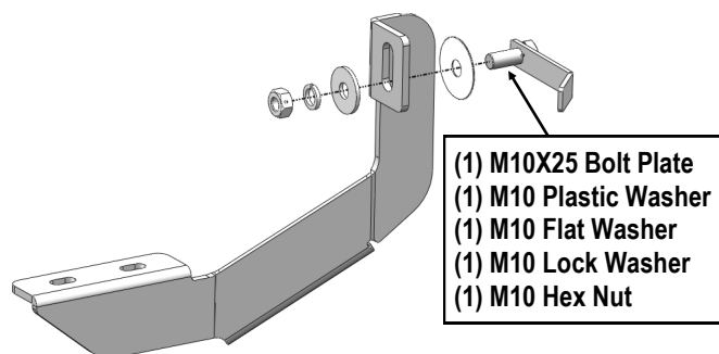
(Fig 10) Passenger Center Mounting Bracket Installation
