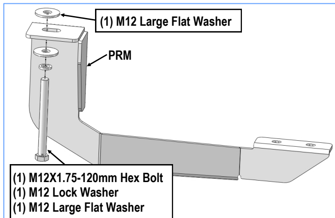
(Fig 11) Passenger Rear Mounting Bracket Installation
