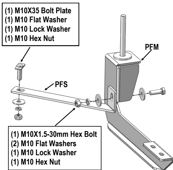
(Fig 7) Passenger Front Brackets Assembly
