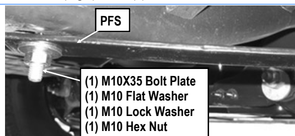
(Fig 6) Passenger Front Support Bracket Installation
