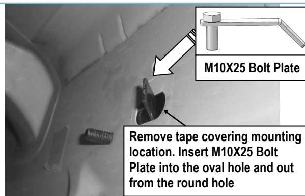
(Fig 8) Passenger Side Center Mounting Location
