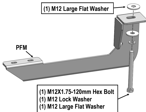
(Fig 4A) Passenger Front Mounting Bracket Installation
