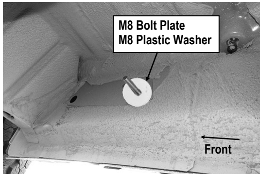
(Fig 13B) Passenger Side Front Mounting Location
