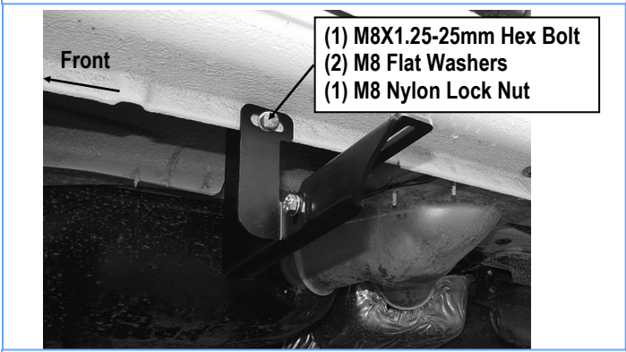
(Fig 12) Driver Side Support Bracket Installed on Pinch Weld
