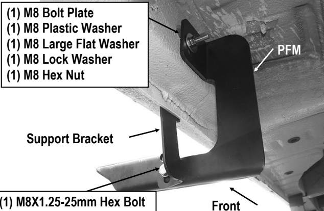
(Fig 13B) Passenger Side Front Mounting Location
