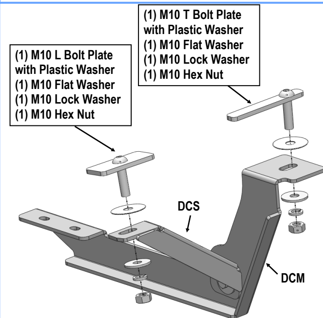
(Fig 14) Driver Side Center Brackets Installed
