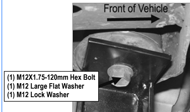
(Fig 6) Driver Side Rear Mounting Bracket (DRM) Installed
