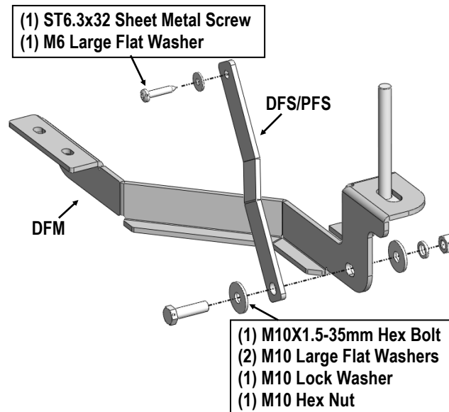
(Fig 3) Driver Front Support Brackets Installation
