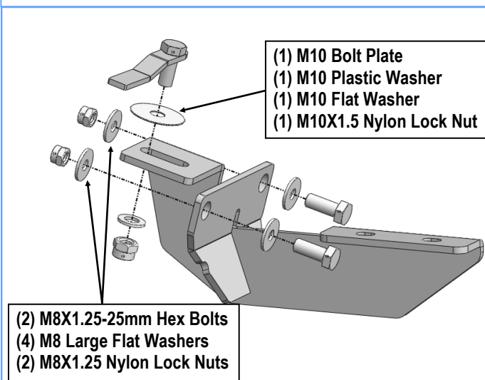
(Fig 3) Driver Front Mounting Bracket Installation
