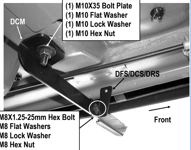
(Fig 7) Driver Side Center Brackets Installed
