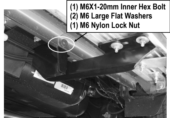
(Fig 15) Support Bracket Installed
