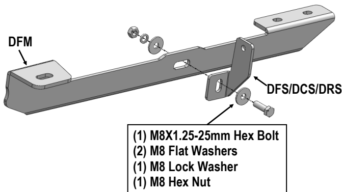
(Fig 2) Driver Front Mounting Bracket Assembly
