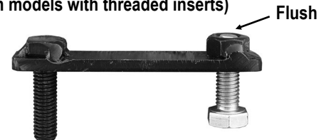
(Fig 3) Thread (1) M8X1.25-30 Hex Bolt into the welded nut on the plate.
