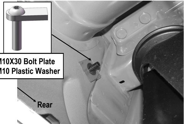
(Fig 14) Insert The M10X30 Bolt Plate
