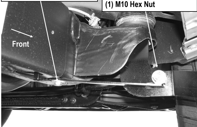
(Fig 7) Passenger Side Front Support Bracket Installed (1500 Models )
