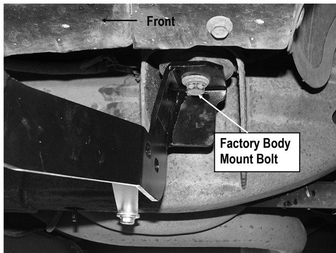
(Fig 5) Passenger Front Mounting Bracket Installed
