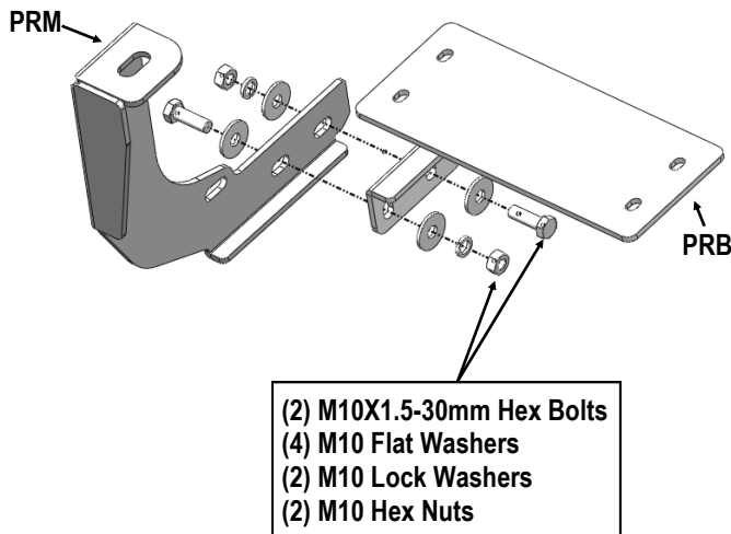
(Fig 11) Passenger Rear Brackets Assembly
