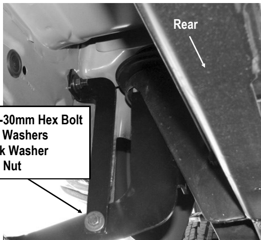
(Fig 16) Passenger Side Rear Support Bracket Assembly
