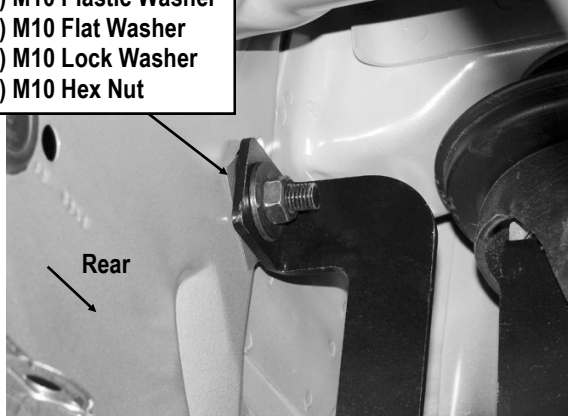
(Fig 15) Passenger Side Rear Support Bracket Installation
