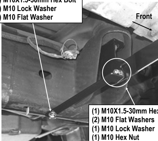
(Fig 8) Passenger Front Support Bracket Installed (Up to 2011 2500/3500 Models )
