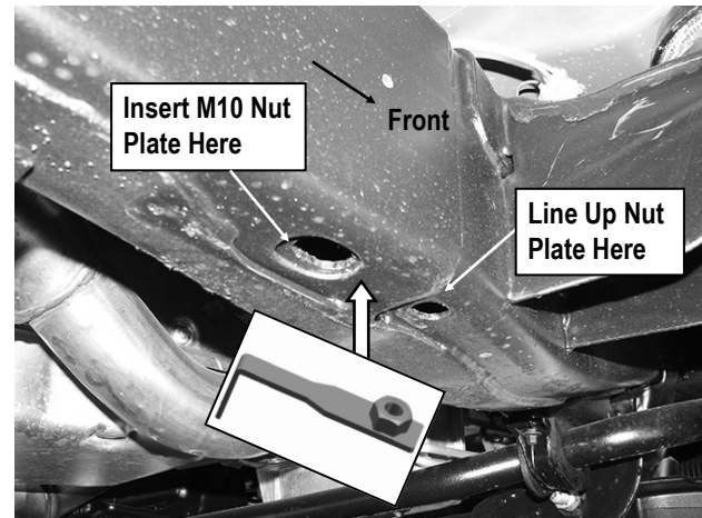
(Fig 6) Passenger Front Support Bracket Mounting Location
