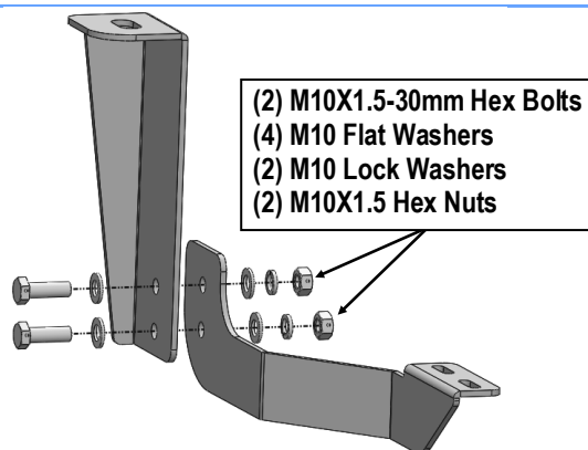
(Fig 8) Passenger Rear Mounting Bracket Assembly
