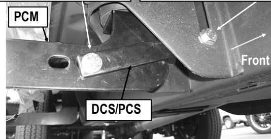
(Fig 6) Passenger Center Bracket Installed (1500 Models)
