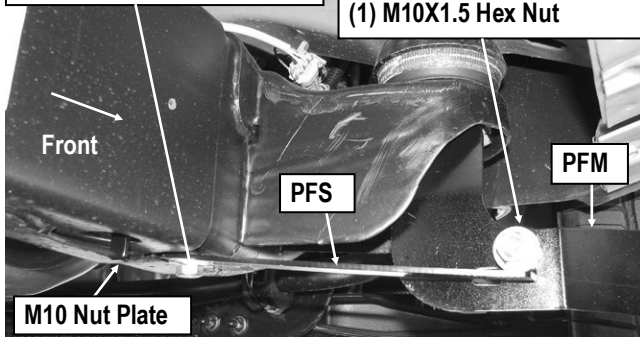
(Fig 4) Passenger Side Front Support Bracket Installed (1500 Models )
