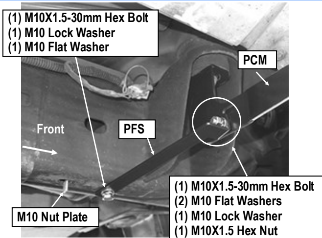
(Fig 5) Passenger Front Support Bracket Installed (Up to 2007 2500/3500 Models )
