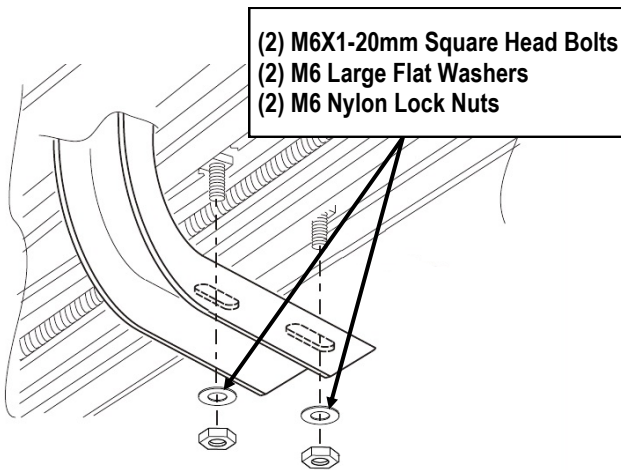
(Fig 7) Running Board Installed Onto Mounting Bracket
