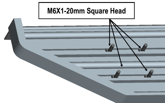
(Fig 6) Slip M6X1-20mm Square Head Bolts Into The Bottom Channels
