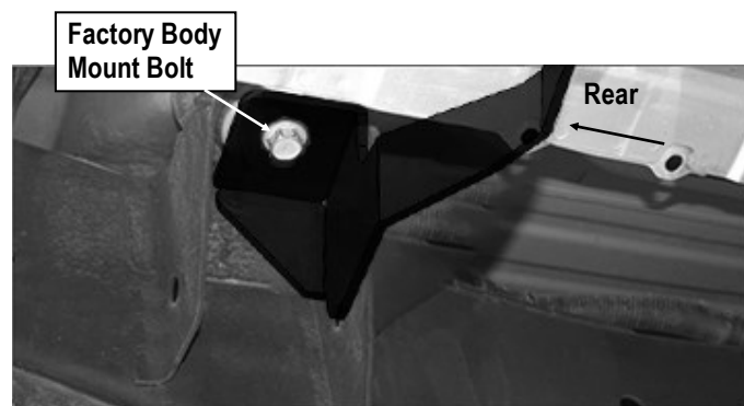
(Fig 8) Passenger Rear Mounting Bracket (PRM) Installation
