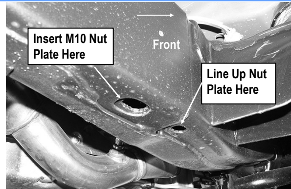
(Fig 3) Passenger Front Support Bracket Mounting Location
