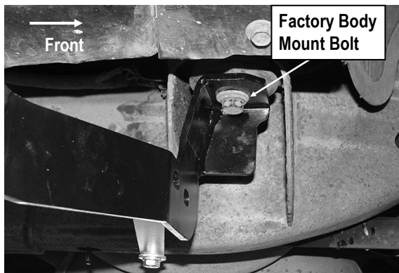
(Fig 2) Passenger Front Mounting Bracket Installed
