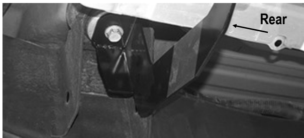
(Fig 9) Passenger Rear Mounting Bracket Installed
