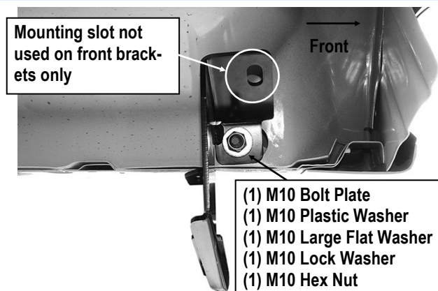
(Fig 7) Driver Front Mounting Bracket (DFM) Installed
