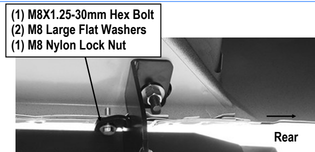
(Fig 22) Attach Passenger Rear Mounting Bracket (The Last One) to Pinch Weld
