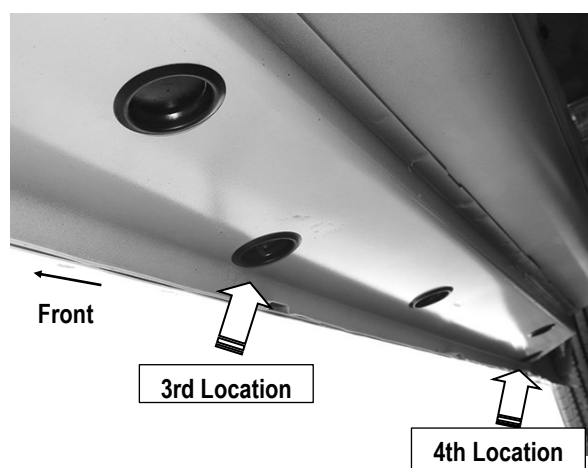
(Fig 17) Passenger Side Rear Mounting Locations
