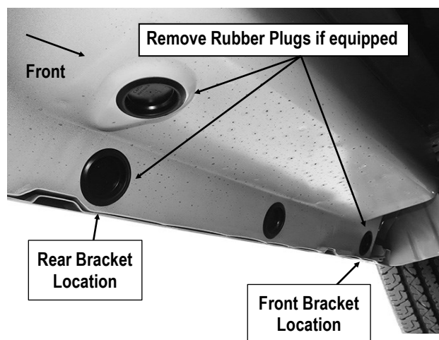
(Fig 4) Driver Side Mounting Bracket Locations
