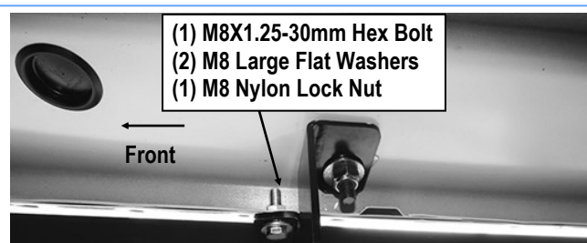
(Fig 21) Attach Passenger Rear Mounting Bracket (the 3rd one) to Pinch Weld
