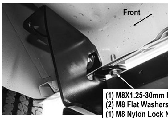
(Fig 19) Attach Passenger Front Mounting Bracket To Pinch Weld
