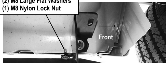
(Fig 12) Attach Driver Front Mounting Bracket To Pinch Weld
