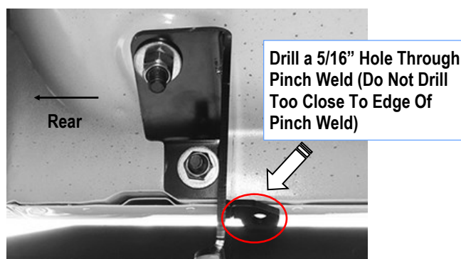
(Fig 11) Driver Hole On Driver Side Rear Mounting Location
