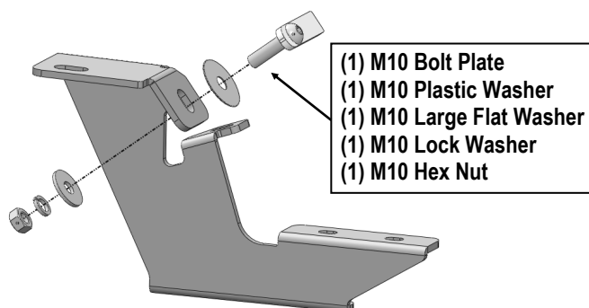
(Fig 6) Driver Front Mounting Bracket (DFM) Installation
