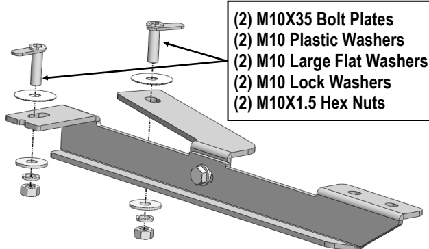
(Fig 5) Driver Side Center Brackets Assembly
