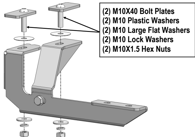
(Fig 9) Driver Side Rear Brackets Installation
