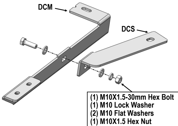
(Fig 5) Driver Side Center Brackets Assembly
