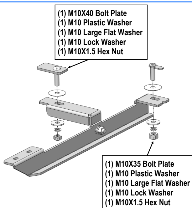
(Fig 3) Driver Side Front Brackets Installation
