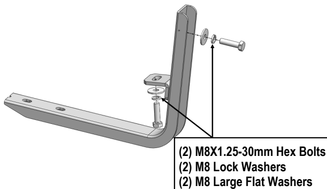
(Fig 7) Driver Front Mounting Bracket Installation
