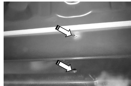
(Fig 5) Driver Side 4th Mounting Location
