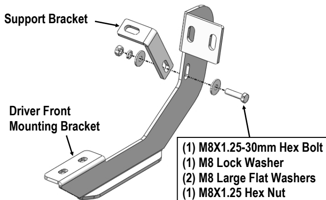
(Fig 1) Driver Front Support & Mounting Bracket Assembly
