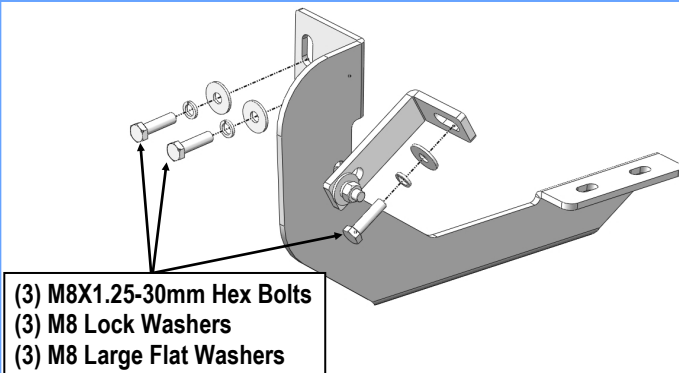
(Fig 2) Driver Front Support & Mounting Bracket Installation
