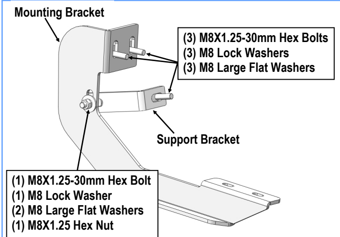
(Fig 3) Driver Rear Support & Mounting Bracket Installation
