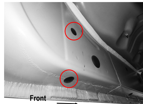
(Fig 5) Driver Rear Mounting Bracket Location
