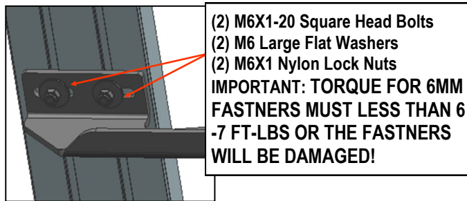
(Fig 11) Running Board Installed Onto Mounting Bracket
