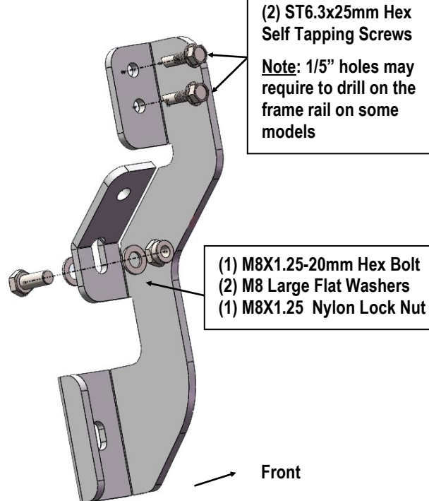
(Fig 2) Driver Center & Rear Mounting Brackets (DCM/DRM) Installation Pictured
