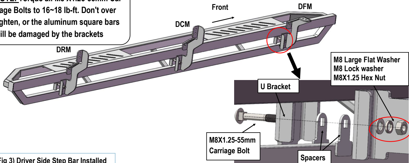
(Fig 3) Driver Side Step Bar Installed
