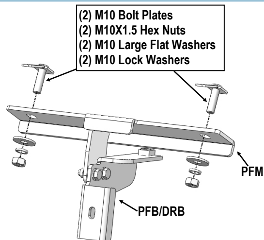
(Fig 5) Passenger Front Mounting Brackets (PFM) Installation
