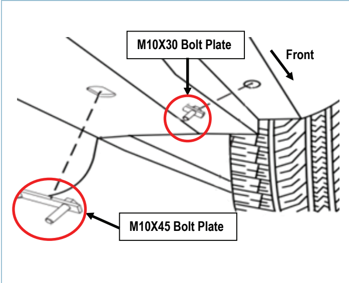
(Fig 1) Passenger Front Mounting Location Pictured
