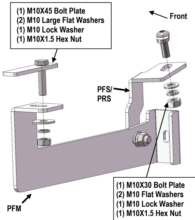
(Fig 3) Passenger Front Mounting Bracket Installation
