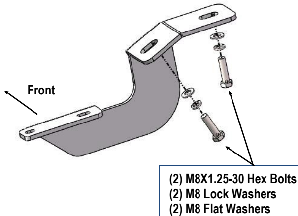
(Fig 2) Passenger Front Mounting Bracket (PFM) Installed
