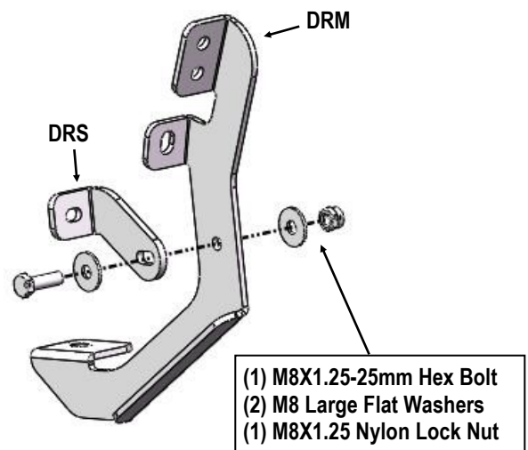
(Fig 3) Driver Side Rear Brackets Assembly
