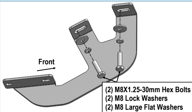
(Fig 2) Driver Front Mounting Bracket (DFM) Installation
