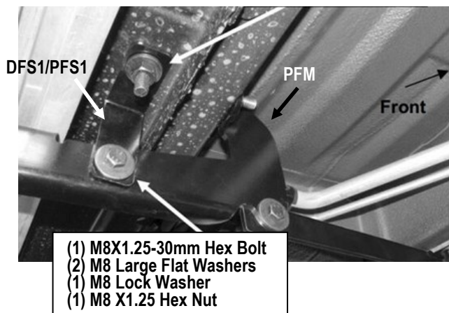
(Fig 8) Passenger Front Mounting Bracket Installed (to the Installed DFS/PFS)
