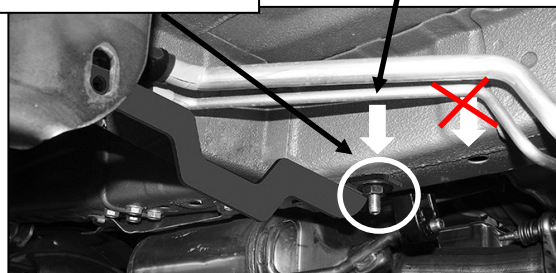
(Fig 10) Passenger Front Long Inner Support Bracket Location
