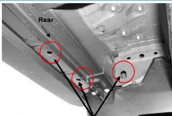
(Fig 12) Passenger Side Rear Mounting Location
