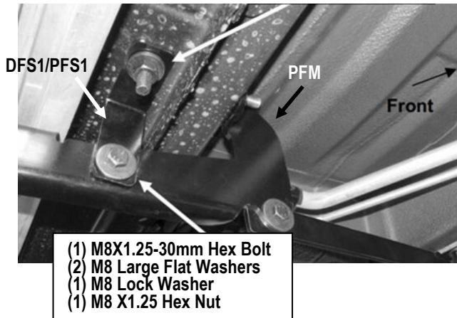
(Fig 8) Passenger Front Mounting Bracket Installed (to the Installed DFS1/PFS1)
