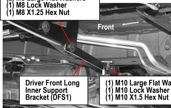
(Fig 11A) Driver Front Long Inner Support Bracket (DFS1) Installed
