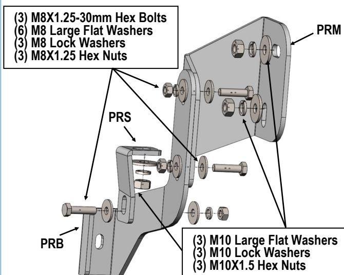
(Fig 19) Passenger Side Rear Brackets Installation
