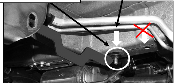
(Fig 10) Passenger Front Long Inner Support Bracket Location
