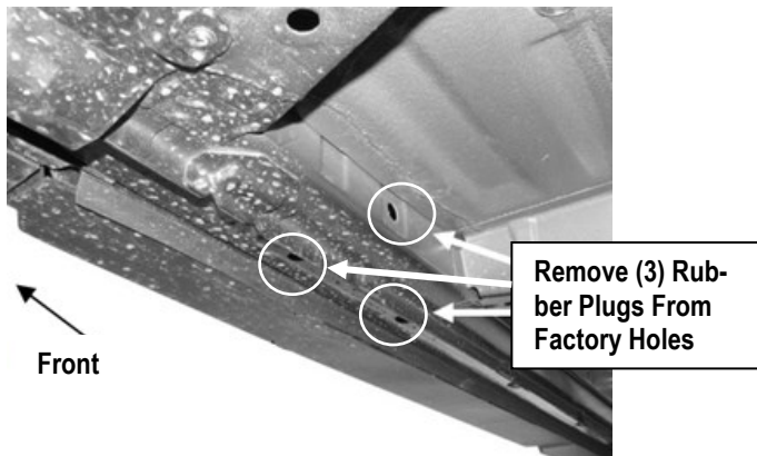
(Fig 1) Passenger Side Front Mounting Location
