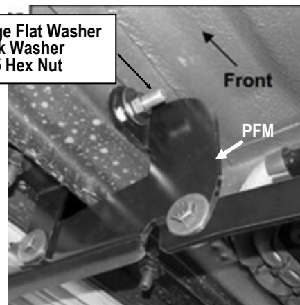
(Fig 7) Passenger Front Mounting Bracket Installed (to the Installed Bolt Plate on Body Panel)
