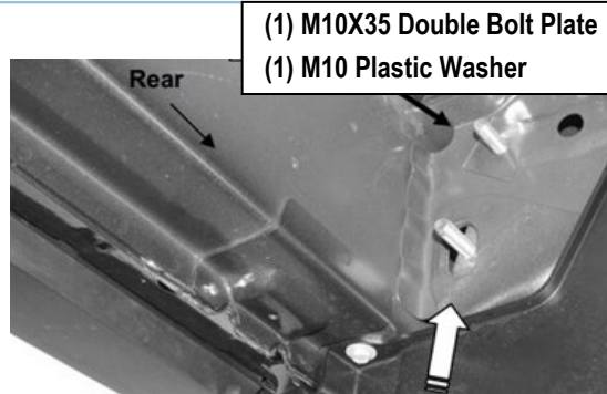
(Fig 13) M10X35 Double Bolt Plate Installed (on Passenger Side Rear Mounting Location)
