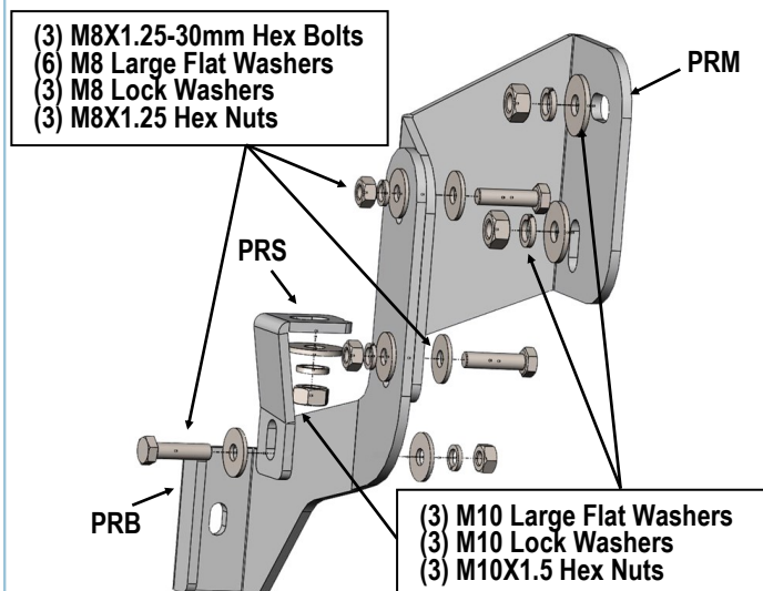
(Fig 19) Passenger Side Rear Brackets Installation
