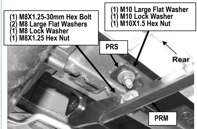
(Fig 18) Passenger Rear "7" Outer Support Bracket (PRS) Installed
