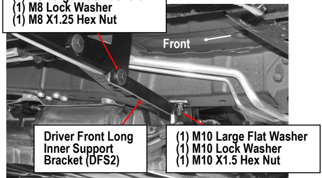
(Fig 11A) Driver Front Long Inner Support Bracket (DRS2) Installed
