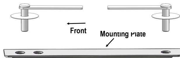
(Fig 3) Mounting Plate Installation (On Passenger Side Front Mounting Location)
