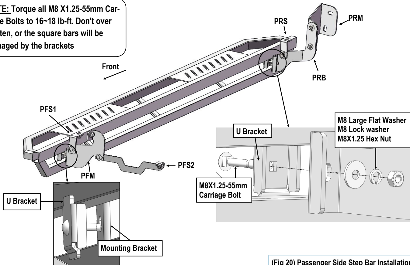
(Fig 20) Passenger Side Step Bar Installation
