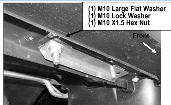
(Fig 4) Mounting Plate Installed (On Passenger Side Front Mounting Location)
