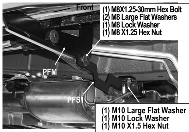
(Fig 11B) Passenger Front Long Inner Support Bracket (PFS1) Installed
