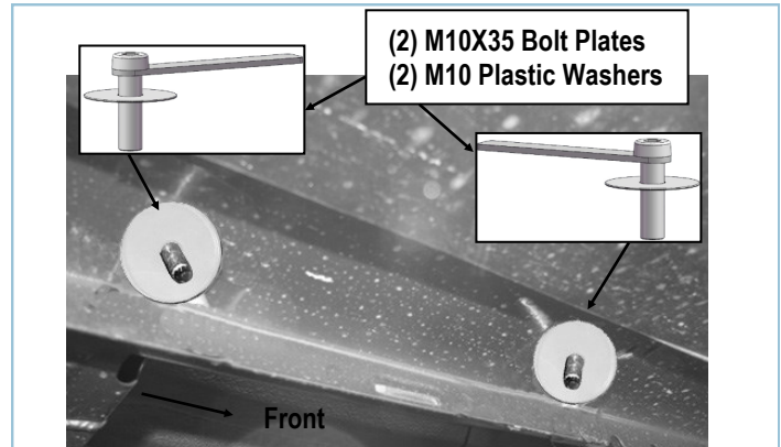
(Fig 2) M10X35 Bolt Plates Installed (On Passenger Side Front Mounting Location)
