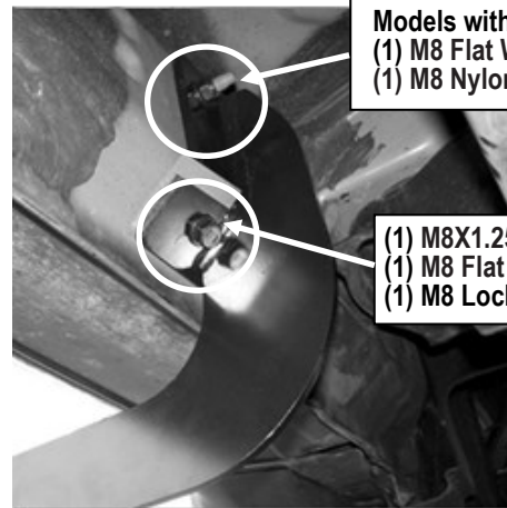
(Fig 3) Driver Front Mounting Bracket Installed
