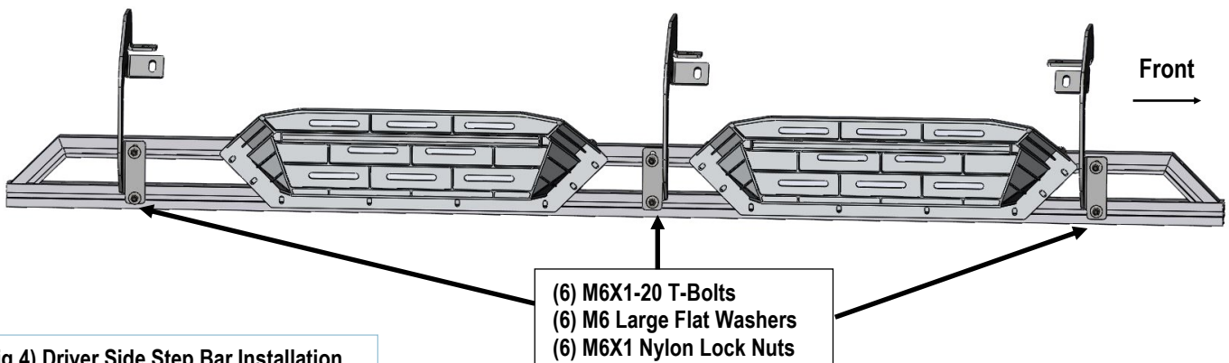
(Fig 4) Driver Side Step Bar Installation
