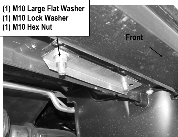
(Fig 4) Mounting Plate Installed (On Passenger Side Front Mounting Location)
