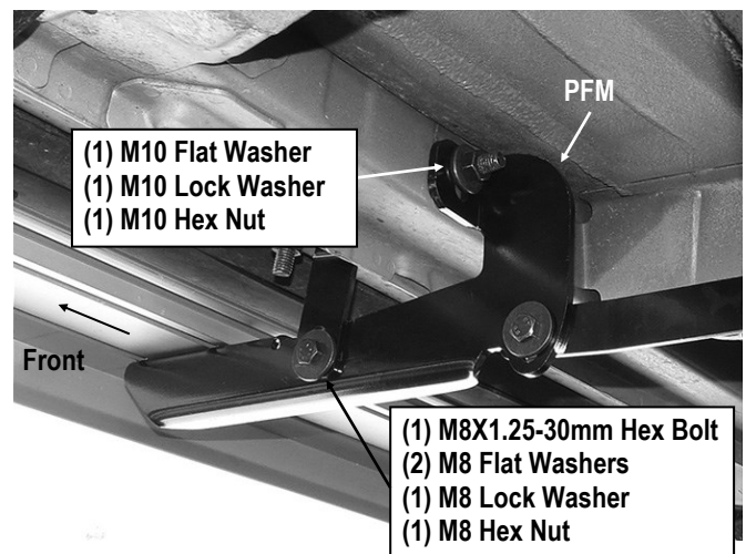
(Fig 7) Passenger Front Mounting Bracket Installed (to the Installed Bolt Plate on Body Panel)
