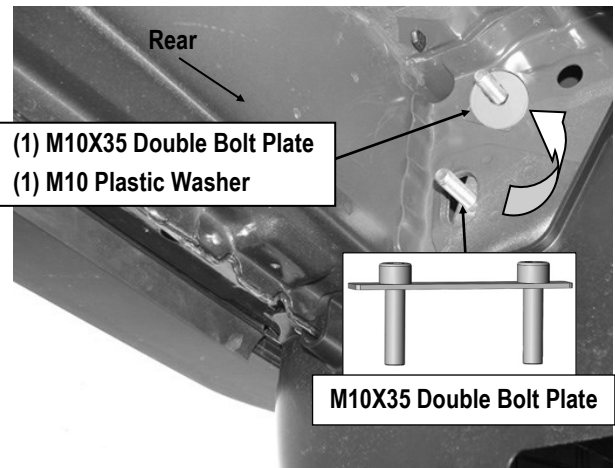
(Fig 14) M10X35 Double Bolt Plate Installed (on Passenger Side Rear Mounting Location )
