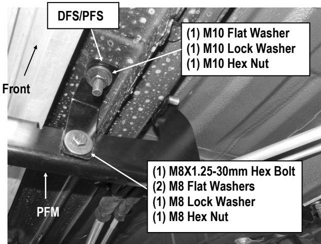
(Fig 8) Passenger Front Mounting Bracket Installed (to the Installed DFS/PFS)
