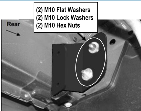
(Fig 17) Passenger Rear Mounting Bracket Installation
