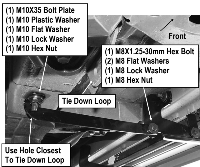
(Fig 11) Driver Front Long Support Bracket (DFS1) Location
