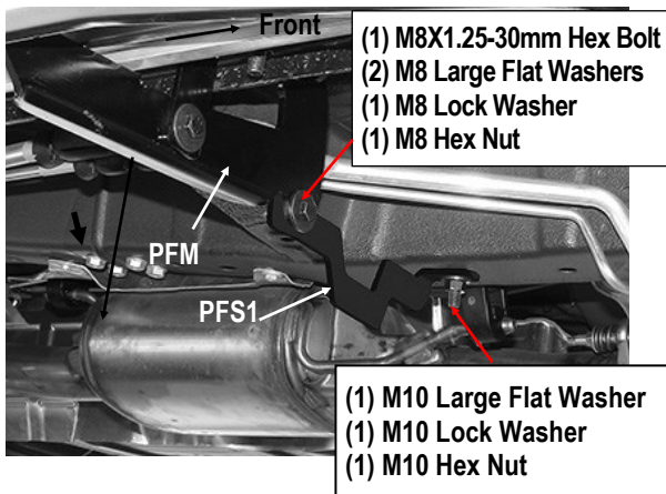
(Fig 12) Passenger Front Long Inner Support Bracket (PRS1) Installed
