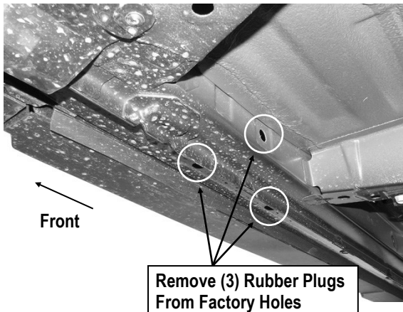
(Fig 1) Passenger Front Mounting Bracket Location
