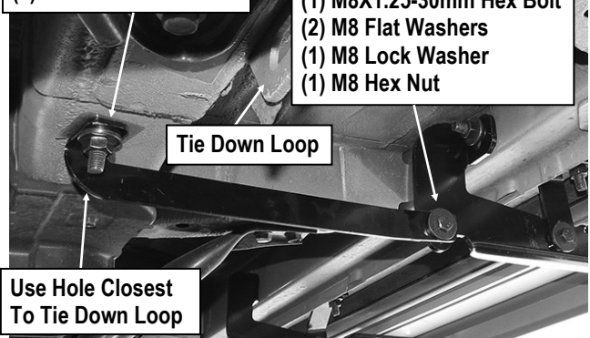
(Fig 11) Driver Front Long Support Bracket (DFS1) Location
